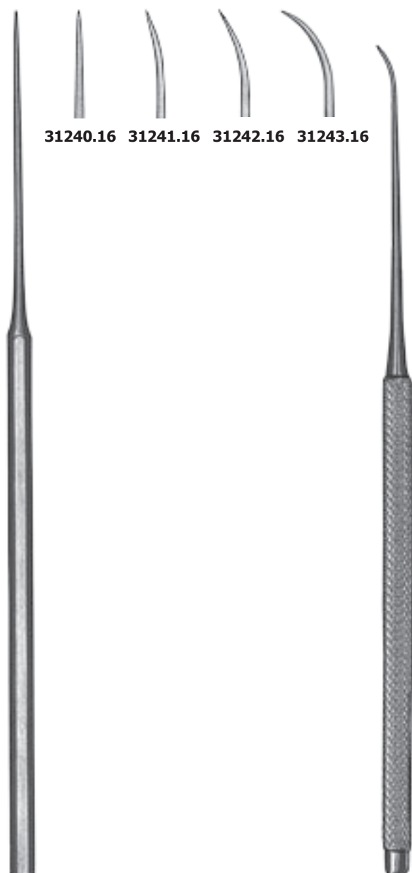
ROSEN Micro Needles round handle sharp 16cm (6¼") 31240.16 RD straight 31241.16 RD very slight curve 31242.16 RD slight curve 31243.16 RD strong curve
